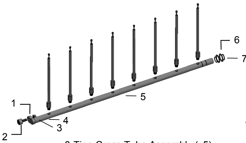
8-Tine Cross Tube Assembly (x5)
