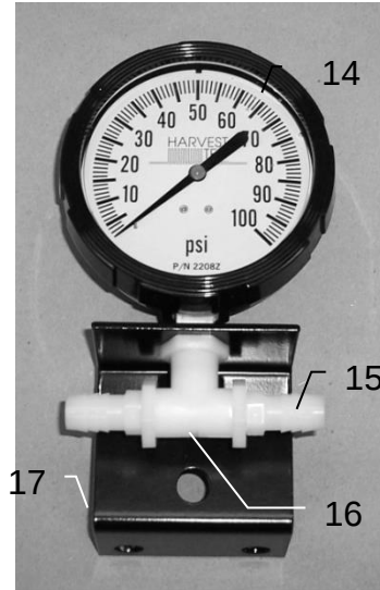
Gauge Assembly for 441
